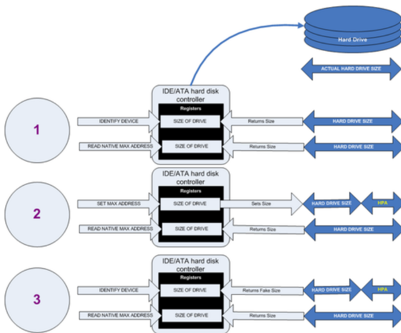
Figure 61: Creation of an HPA
