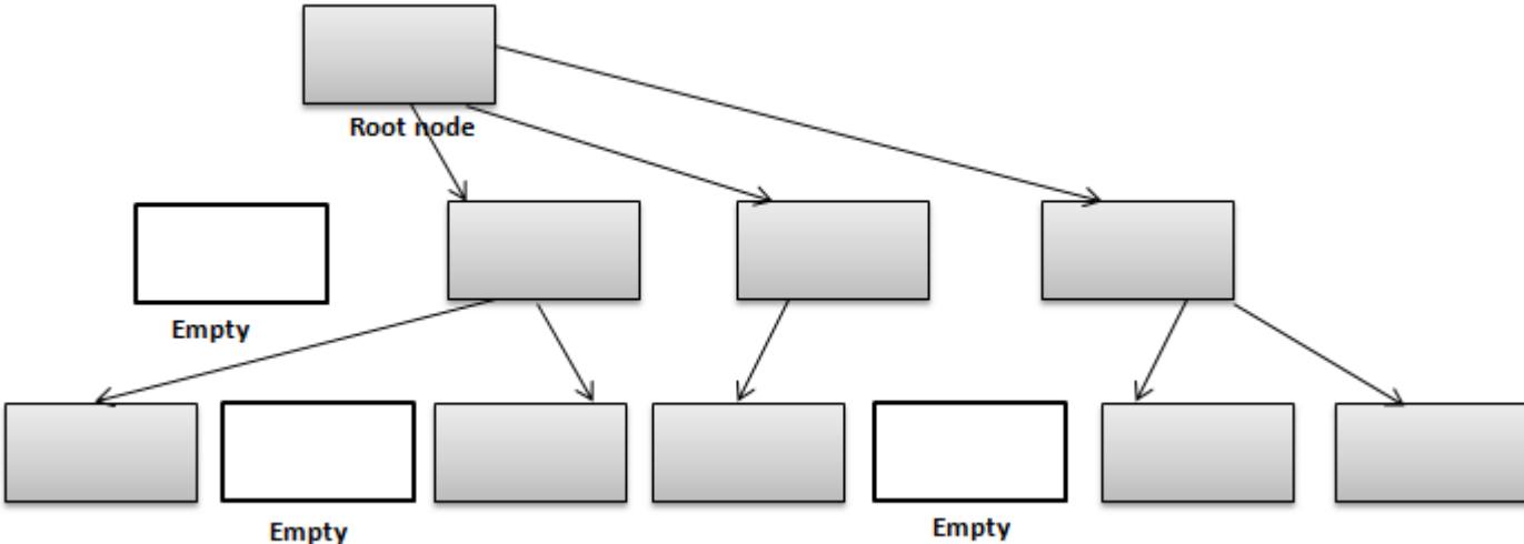
Figure 54: B-tree Structure
