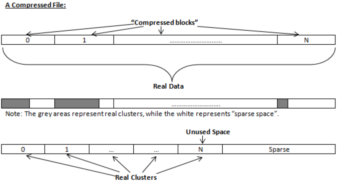
Figure 50: Compressed File Structure
